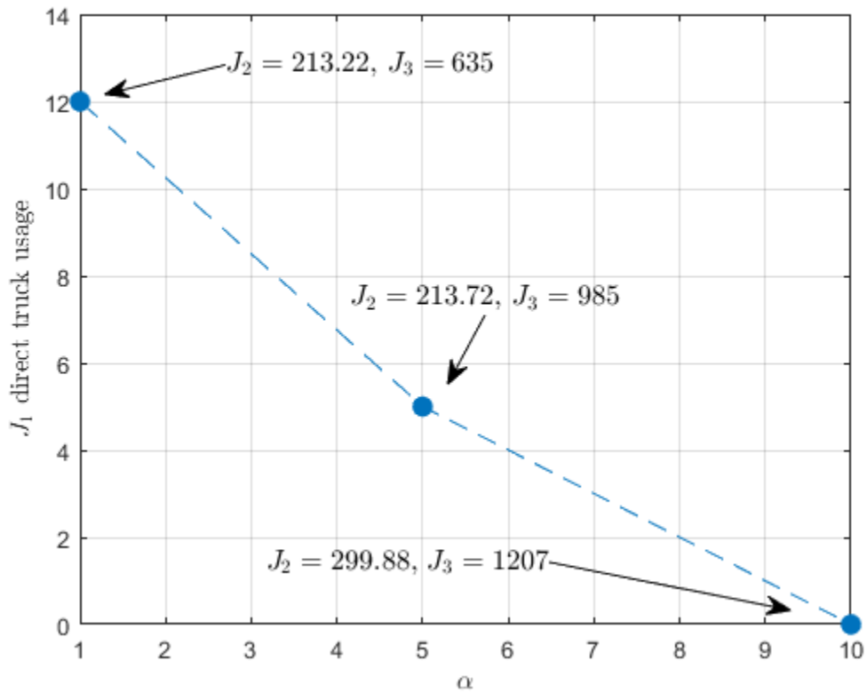
Figure 5. Variation of the objectives as a function of the first objective coefficient.
