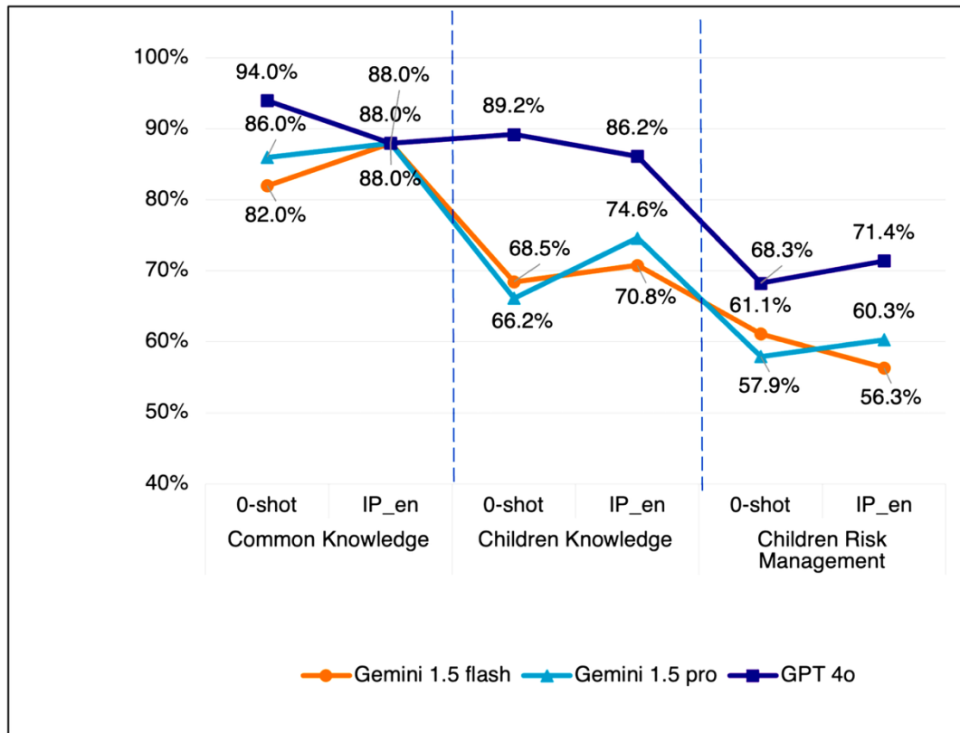
Figure 4. Performance comparison of three LLMs across different multimodal input datasets
