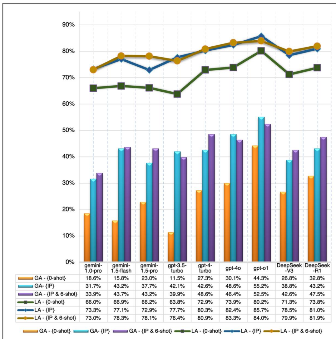
Figure 3. Global accuracy (GA) and local accuracy (LA) of the MulAns dataset
