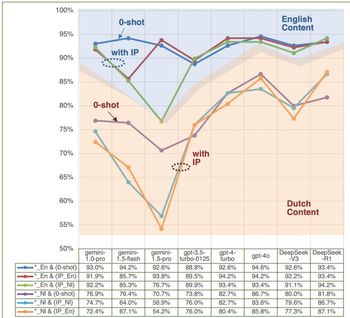
Figure 1. Performance comparison of eight LLMs across two different languages in content and instructional prompts
