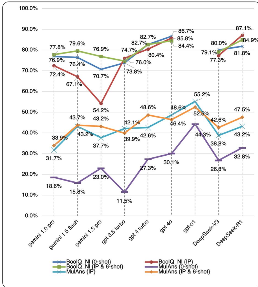
Figure 2. LLM's Performance comparison across different text datasets
