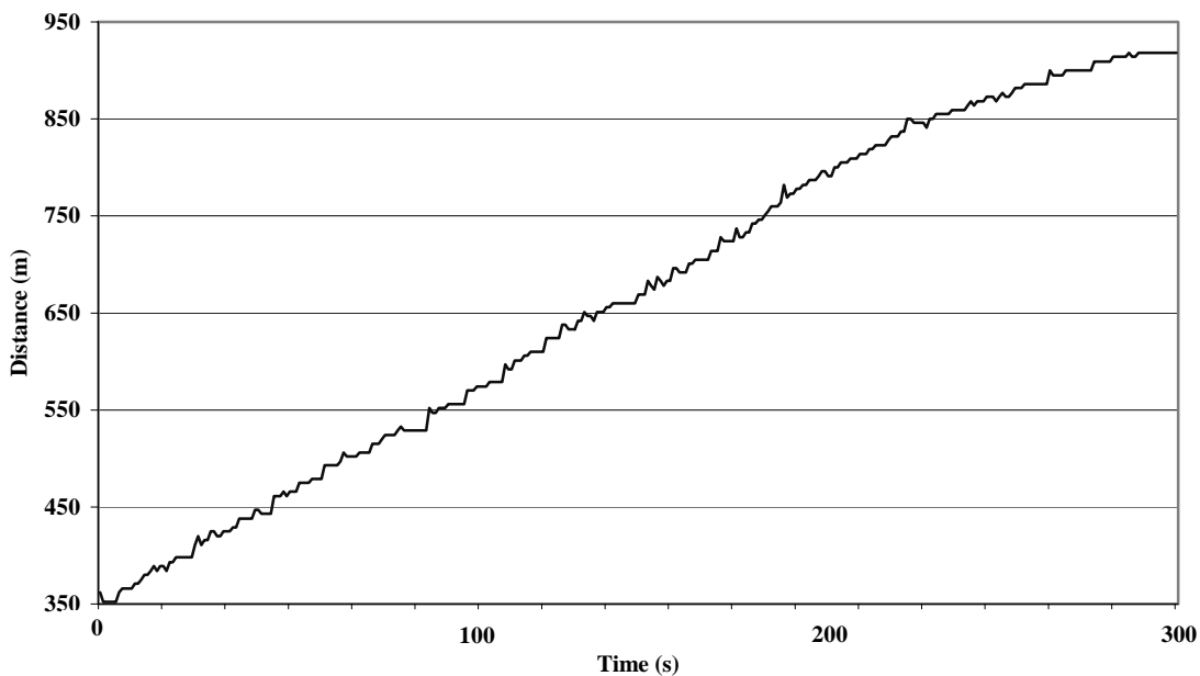
Figure 6. Test line of the Paris metro: Measured distance versus time
