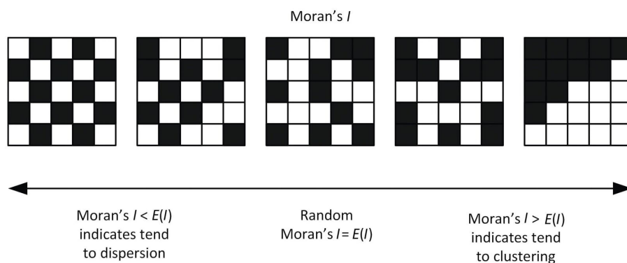
FIG. 5.3 Illustration of how map clustering affects Moran's I score. The Moran's I score, an indicator for spatial clustering, was used to measure the degree of spatial clustering for waste reuse. The Moran's I score ranges from -1 to 1. A value approaching 1 indicates strong spatial clustering, -1 indicates strong spatial dispersion, and 0 indicates the absence of large clusters. Image adapted from (Kirkegaard, 2015).
