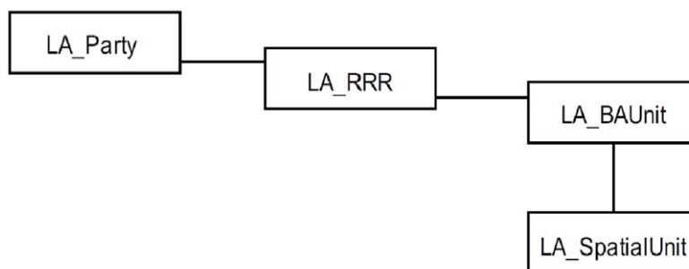
FIG. 2.31 Core classes of the LADM (ISO 19152: 2012)
