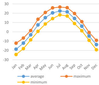
e. Monthly dry bulb temperature (°C), Harbin
