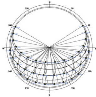
d. Sun path, Harbin
