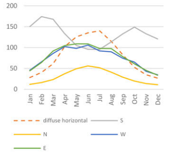
f. Monthly solar radiation (kWh/m2-day), Harbin
