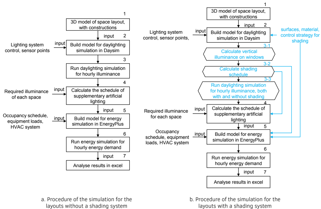
FIG. 3.3 Procedure to integrate daylighting simulation with energy simulation
