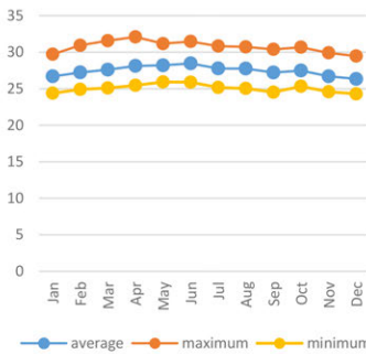
h. Monthly dry bulb temperature (°C), Singapore
