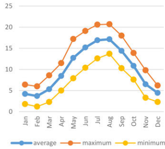
b. Monthly dry bulb temperature (°C), Amsterdam
