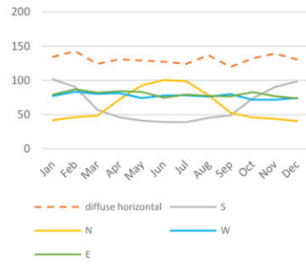
i. Monthly solar radiation (kWh/m2-day), Singapore
