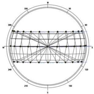
g. Sun path, Singapore
