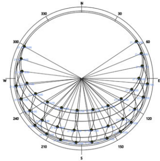
a. Sun path, Amsterdam
