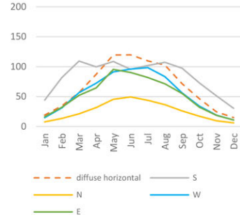
c. Monthly solar radiation (kWh/m2-day), Amsterdam
