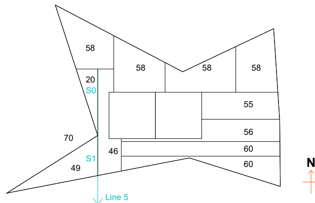
FIG. 5.4 Ignored scenario for splitting the layout. Note: The numbers (m 2 ) in the layout are the corresponding room areas
