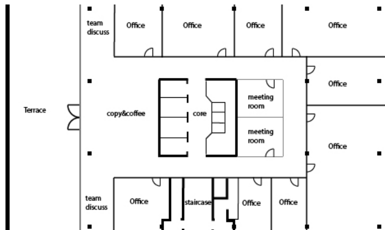
FIG. 3.1 Space layout of the reference building, adapted from [20]
