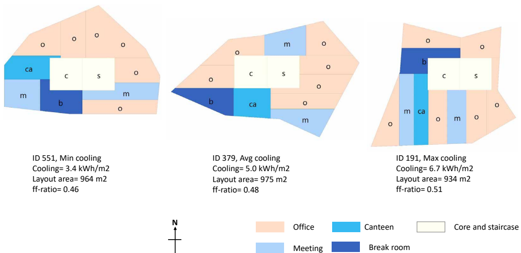
FIG. 5.14 The layout with the minimum cooling demand, the layout with the moderate cooling demand, and the layout with the maximum cooling demand, resulting from the optimisation for minimising cooling demand
