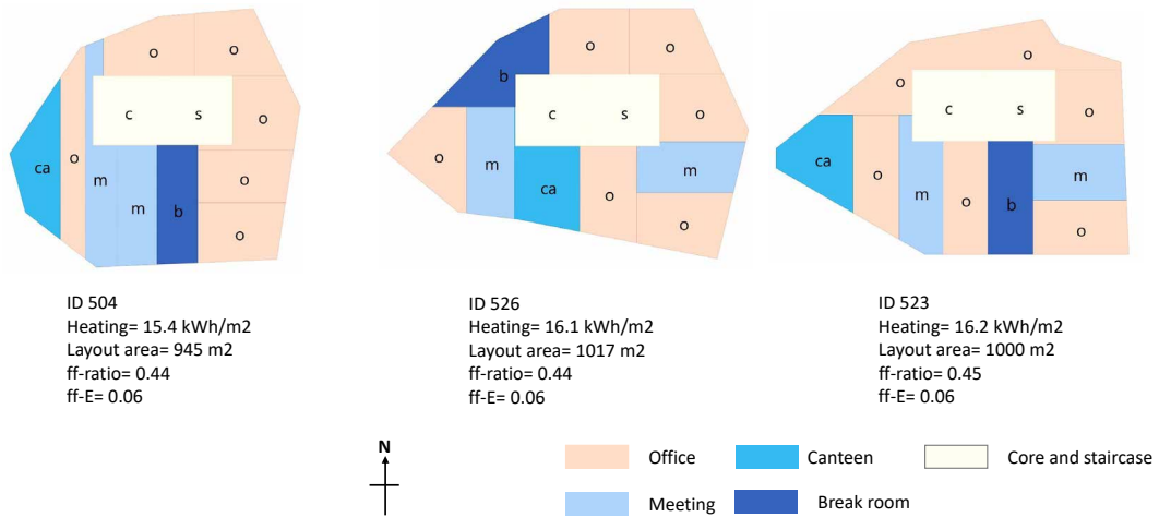
FIG. 5.13 Layouts in which no room orients the West and satisfy layout area constraint, resulting from the optimisation for minimising heating demand Note: The room orientations follow the orientation definition based on the normal of internal walls as Figure 5.5-a shows
