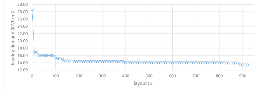
c History chart for minimising heating demand
