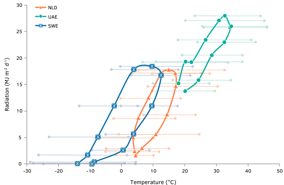
FIG. 3.2 Average daily radiation per month (MJ m -2 d -1 ) and monthly average, minimum and maximum temperatures (°C) for Kiruna (SWE, stars), Amsterdam (NLD, triangles) and Abu Dhabi (UAE, circles). January is the lower left data point in each cycle.
