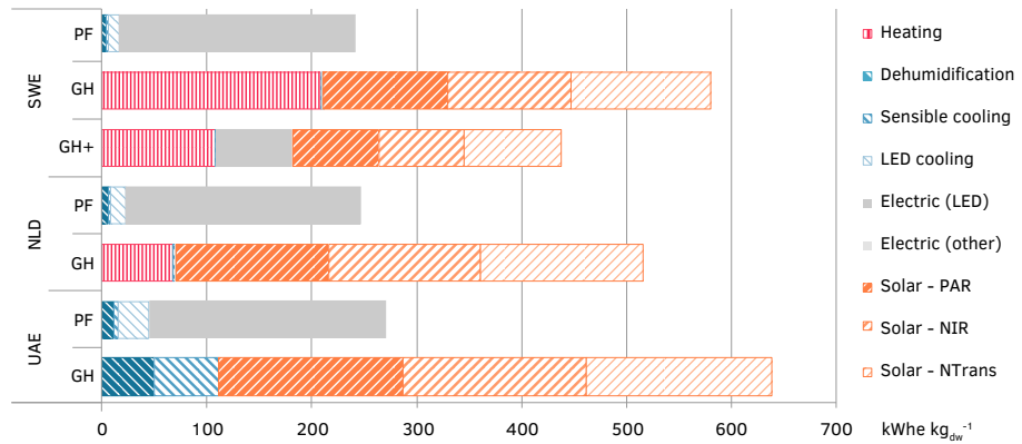
FIG. 3.5 Electricity use per kg lettuce dry matter production ( \text{kWh}_e \text{kg}_{dw}^{-1} ) by end use. Electricity use has been calculated according to the methods described in Section 3.2.4.2.
