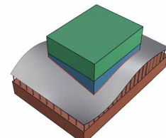
FIGURE 5.8 Casting the foam mould on the flexible table.
