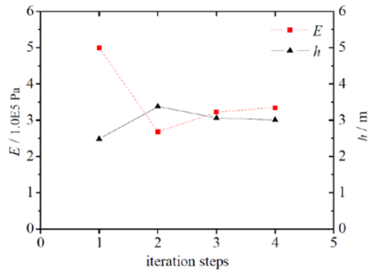
FIGURE 6.3 Iteration curve of Example 6.1.
