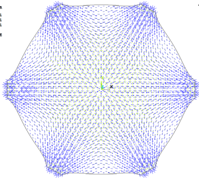
FIGURE 5.23 Vectorial representation of the principal stresses of the shell of Example 5.2 .
