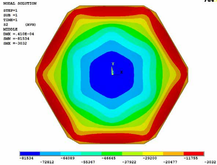
FIGURE 5.52 Principal stress S_2 at the middle surface of the shell of Example 5.4 (Pa).
