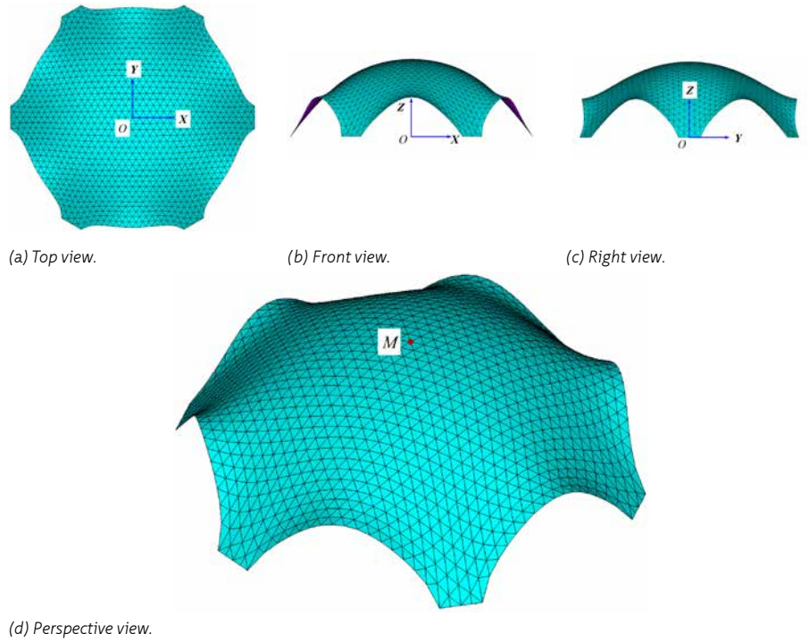
FIGURE 6.4 Form-Control result of Example 6.1.
