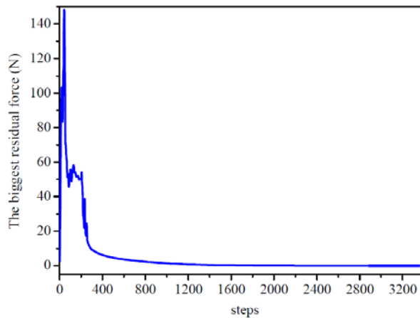
FIGURE 5.32 Evolution curve of the VFIFE method of Example 5.3 .
