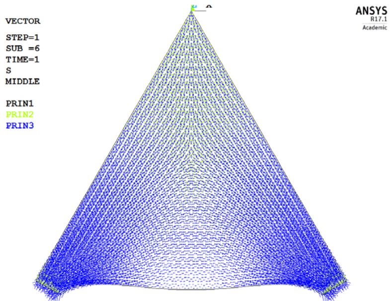
FIGURE 8.32 Vectorial representation of the principal stresses for Model A_s (shell with simply supported straight supports) when the shell fails.
