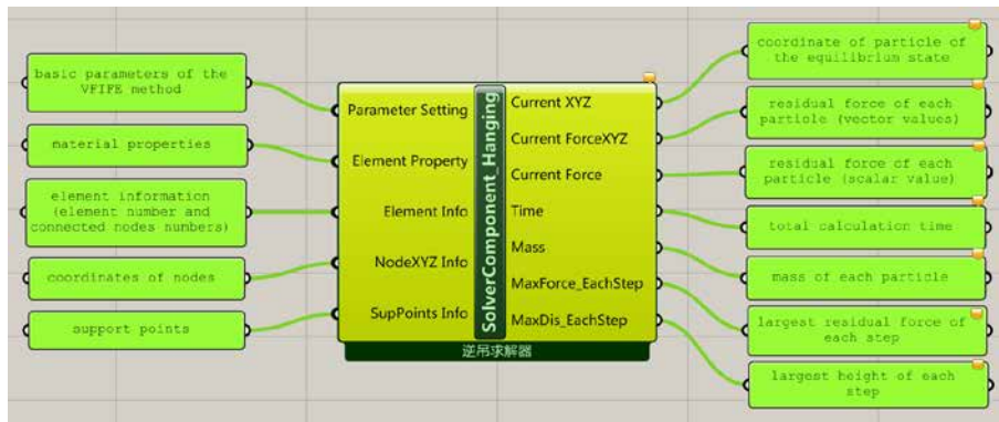
FIGURE 6.20 The calculation component of the plug-in.
