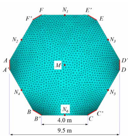
FIGURE 6.12 Initial conditions of Example 6.3 .
