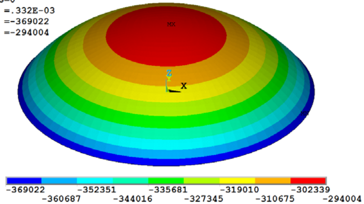
FIGURE 4.12 Principal stress S_3 at the middle surface of the dome (Pa).
