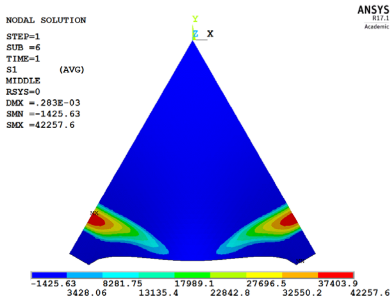
FIGURE 8.24 Principal stress S_1 at the middle surface of Model A 5 (shell with simply supported straight supports; Pa).
