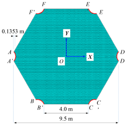
FIGURE 8.13 Initial conditions of Model C (shell with inward-curved supports).
