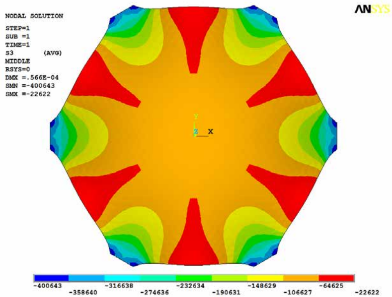
FIGURE 5.22 Principal stress S_3 at the middle surface of the shell of Example 5.2 (Pa).
