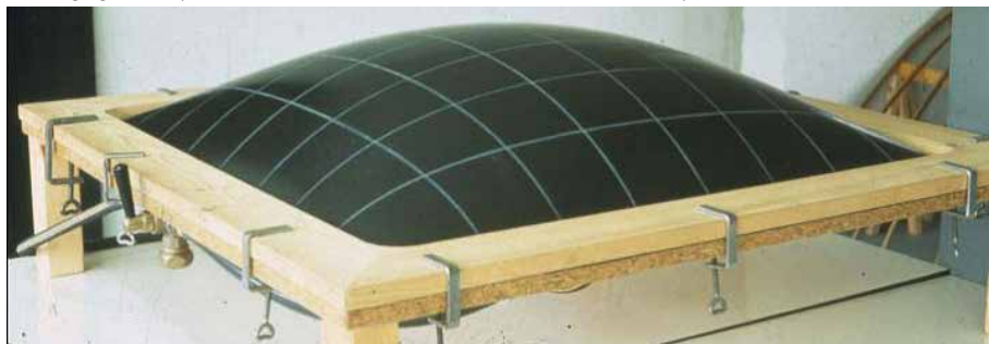
(c) Pneumatic model of Heinz Isler [68].
