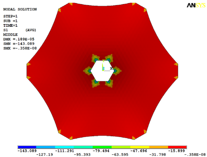
FIGURE 5.37 Principal stress S_1 at the middle surface of the shell of Example 5.3 (Pa).
