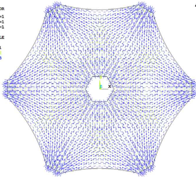
FIGURE 5.40 Vectorial representation of the principal stresses of the shell of Example 5.3 .
