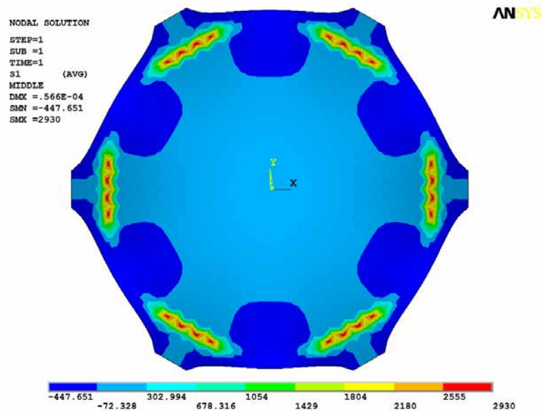
FIGURE 5.20 Principal stress S_2 at the middle surface of the shell of Example 5.2 (Pa).
