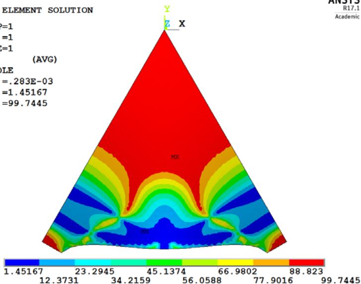
FIGURE 8.22 R_1 of Model A_5 (shell with simply supported straight supports; %).
