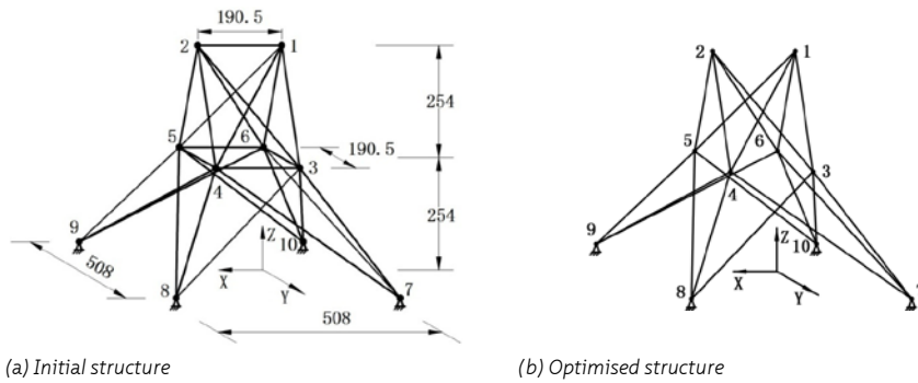
FIGURE 3.13 Size and topology optimisation of the 25-bar spatial truss structure [88].
