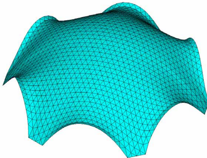
(a) First initial structural system with 2 times the loads in the upper part and its Form-Finding result.
