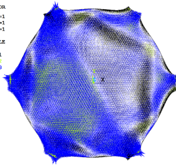
FIGURE 8.37 Vectorial representation of the principal stresses for Model A s (shell with simply supported straight supports) under half-span loads.
