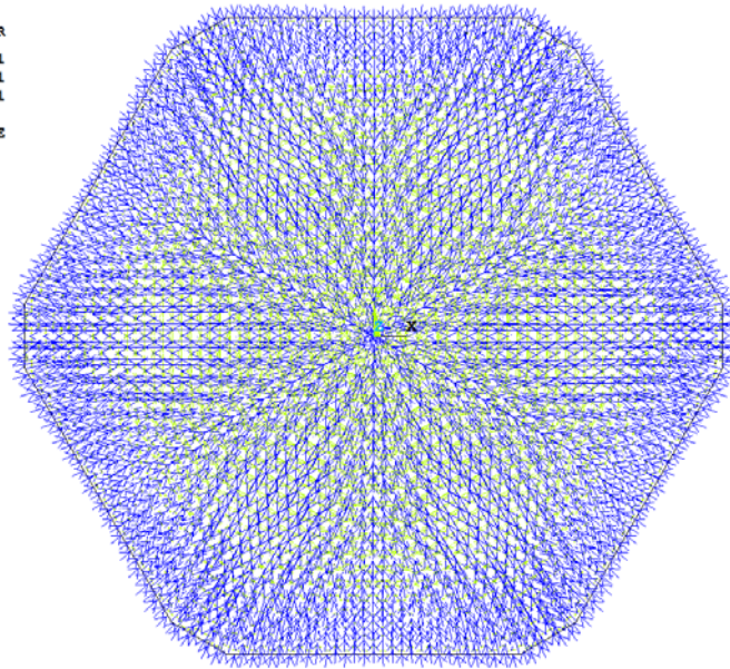
FIGURE 5.54 Vectorial representation of the principal stresses of the shell of Example 5.4 .
