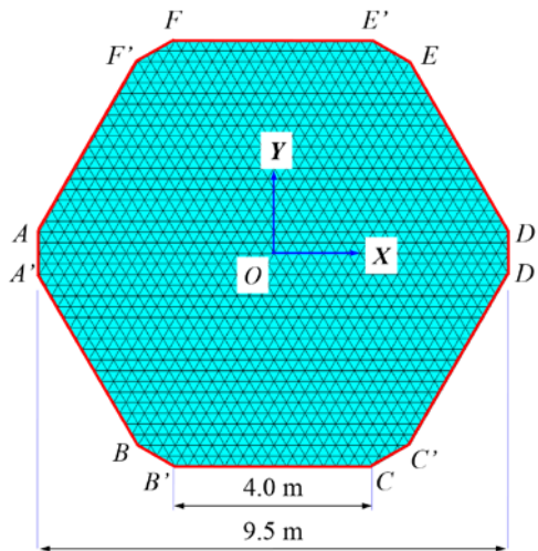
FIGURE 5.45 Initial conditions of Example 5.4 .
